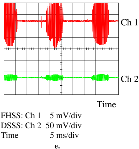
Fig. 8. Interference impact for wireless LANs from model B commercial microwave oven Upper trace represents IEEE 802.11 FHSS, lower trace represents IEEE 802.11 DSSS. Because FHSS is about 20 dB more sensitive for in-band CW interference (at lower risk of true in-band CW), the channel input of the oscilloscope is made 10 times more sensitive for fair comparison.
